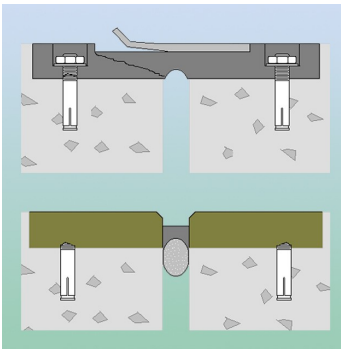
Spalled Joint Face Repair
